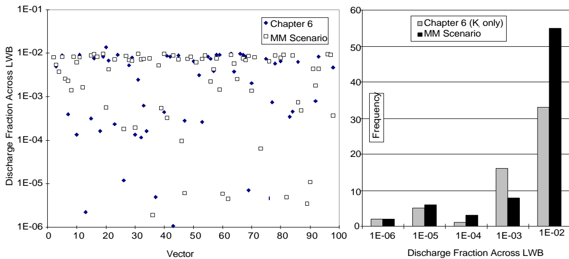
Figure 8.7. Left) Plutonium Fractional Discharge across the LWB for Chapter 6 Results (Full Mining) and MM Scenario with both having 1% of the Initial Mass with a K_d=0 \text{ml/g} Right) Frequency Distribution of both Mining Scenarios for Vectors with Significant Discharge across LWB
